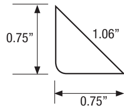
3/4" CHAMFER
